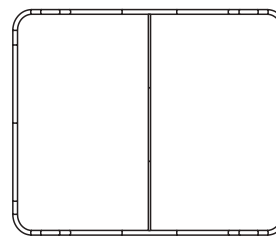
6ft: Front View 1864mm × 1530mm
